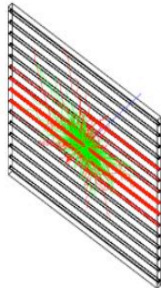
WaveLengthShifting
