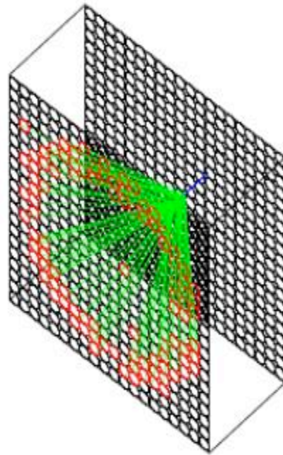
Cerenkov
